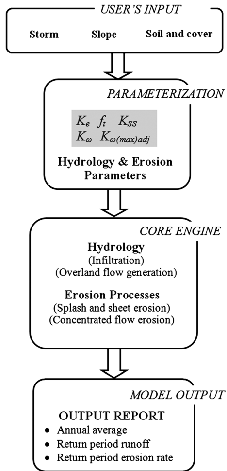
Figure 1. A flow chart of RHEM erosion prediction procedure
